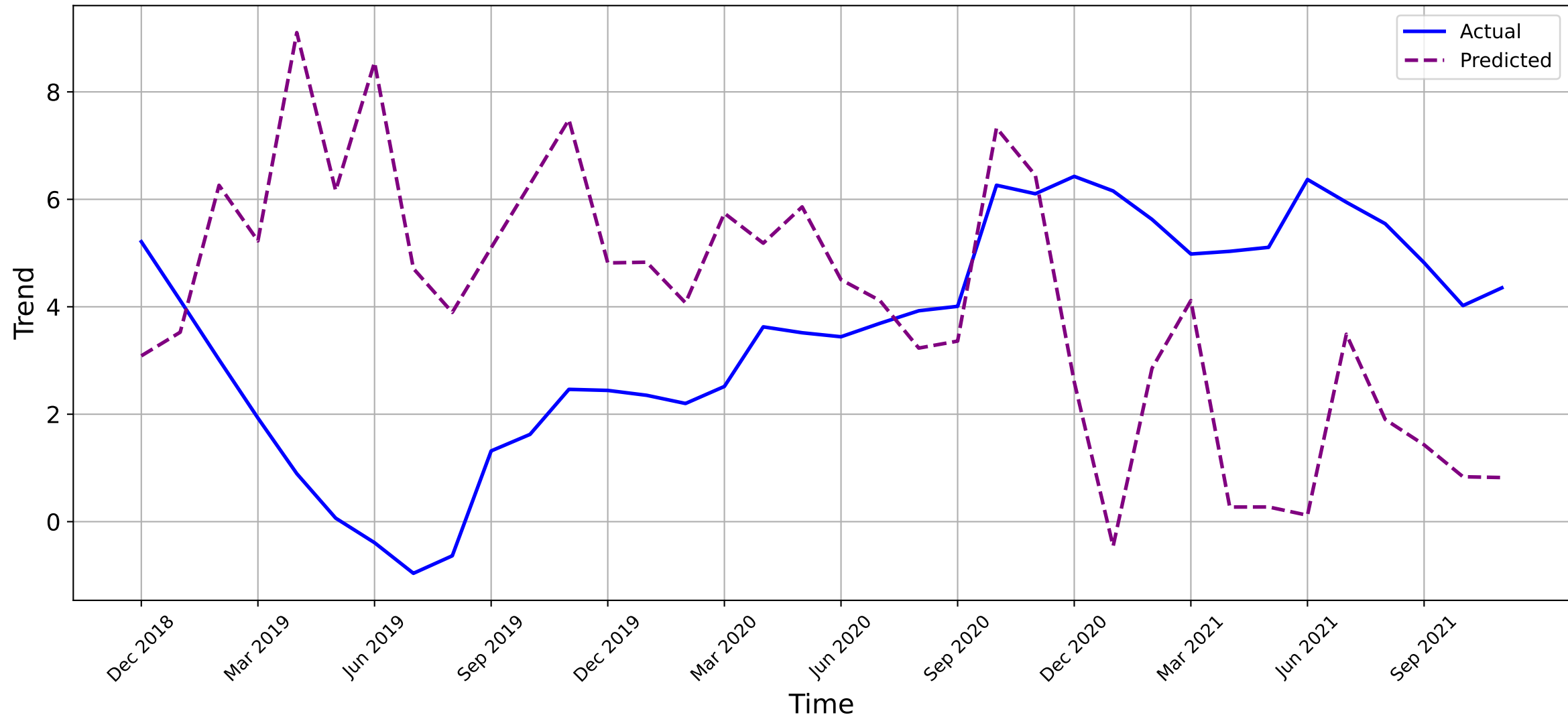
Solution_DNSSEC_Mentions - Validation
